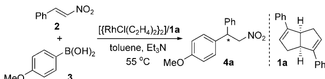
Scheme 1. Initial attempts on using bicyclo[3.3.0] diene ligand.
